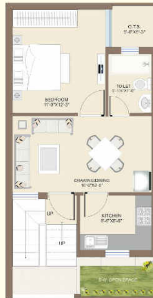
Ground Floor Super Area 630 sq. ft.
