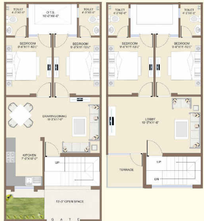
Ground Floor Super Area 900 sq. ft.
