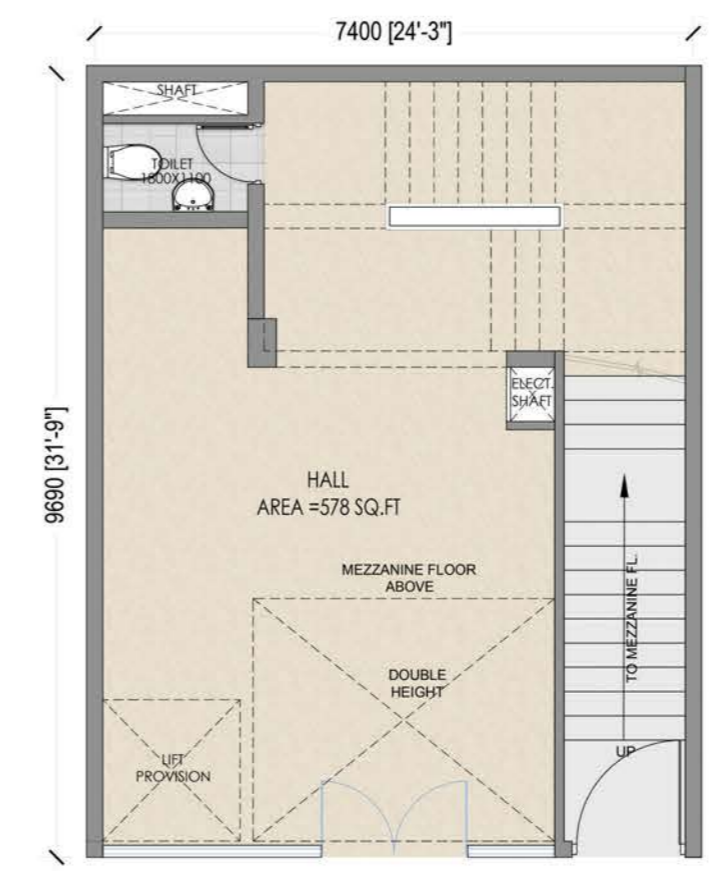
SCO GROUND FL. PLAN
